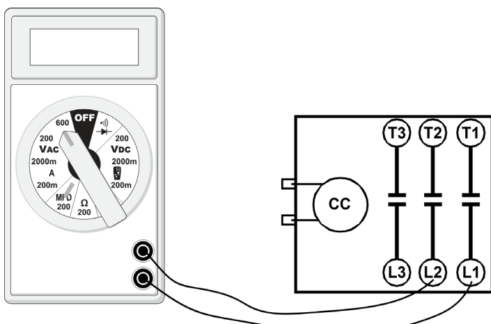
— Voltmeter for testing contacts TESTING COMPRESSOR CONTACTOR (THREE-PHASE)
