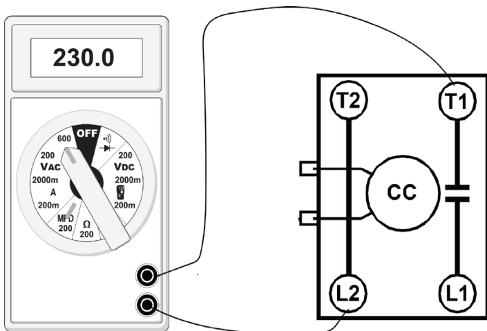
TESTING COMPRESSOR CONTACTOR (SINGLE PHASE)
