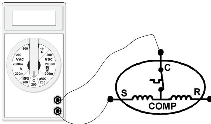
TESTING COMPRESSOR WINDINGS
