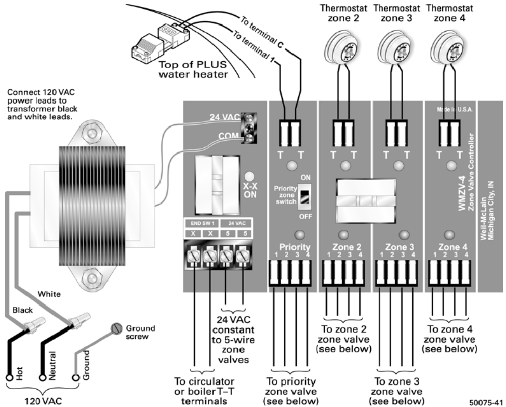
Domestic water priority with Weil-McLain WMZV Zone Valve Controller
