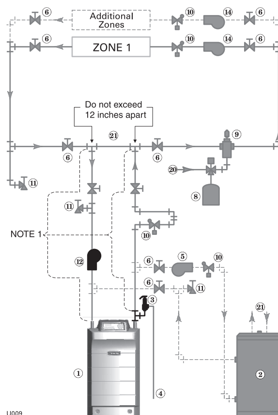
Figure 13 Circulator zoning plus optional water heater piping
