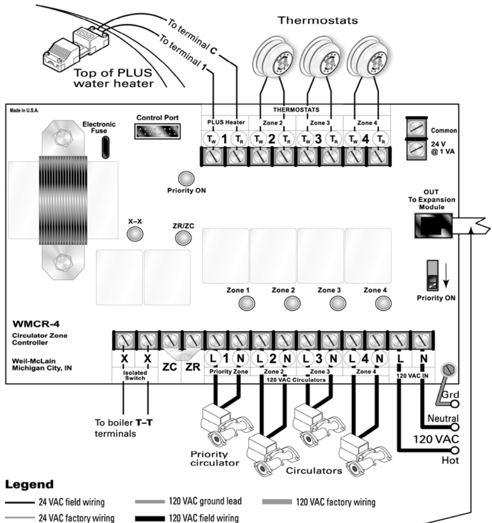
Domestic water priority with Weil-McLain WMCR Circulator Zone Controller
