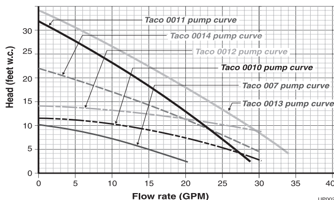
Figure 16 Pump curves for Taco circulators
