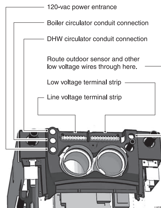
Figure 18 Routing field wiring
