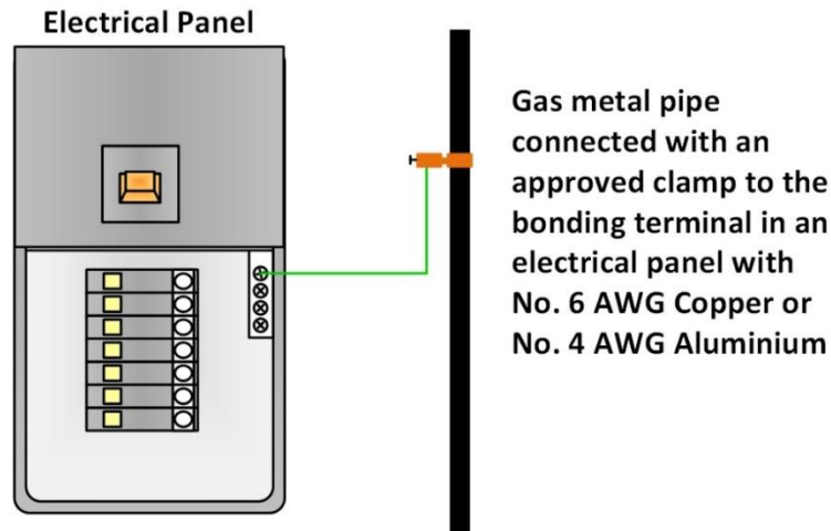
Diagram 8 – Approved pipe clamp with a bonding conductor connected to a bonding bar in an electrical panel
